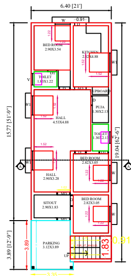
PROPOSED GROUND FLOOR PLAN
