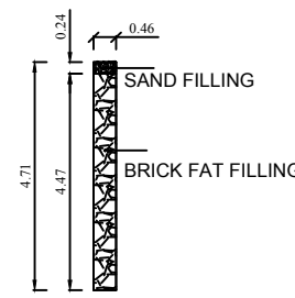
DETAILS OF PERCULATION PIT
