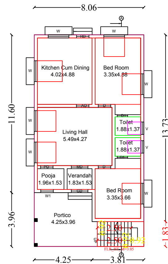
Floor - Ground
