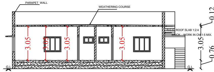
Section on-"AA"
