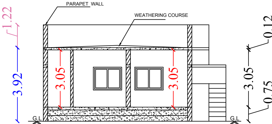
Section on-"AA"
