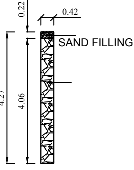
DETAILS OF PERCULATION PIT
