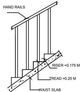
STAIR CASE DETAILS
