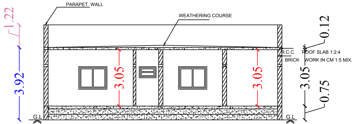
Section on-"AA"
