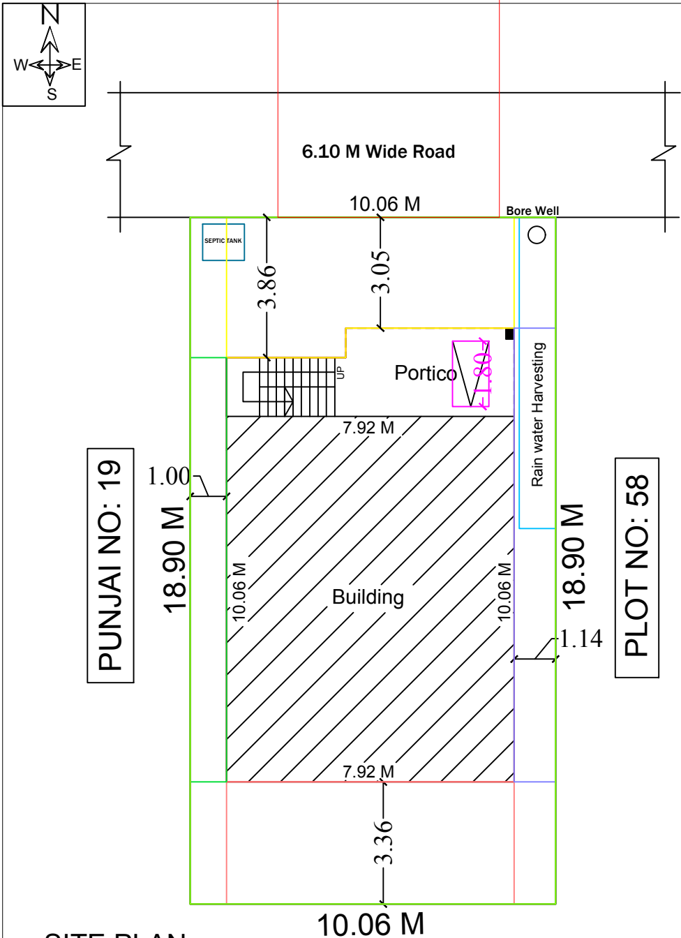
SITE PLAN
