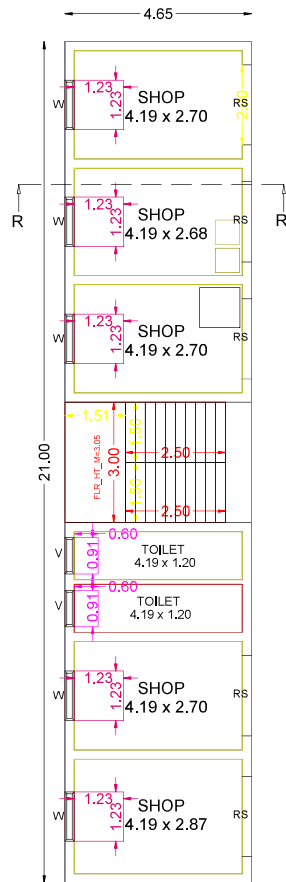
Pro.Ground Floor Plan
