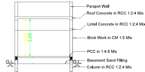
Section RR
