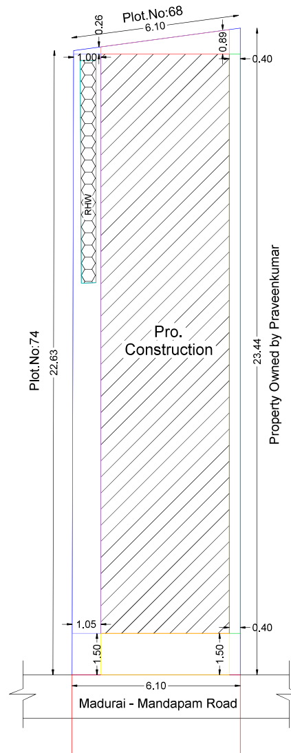
Site Plan
