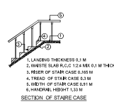
Section RR
