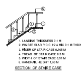
Section RR
