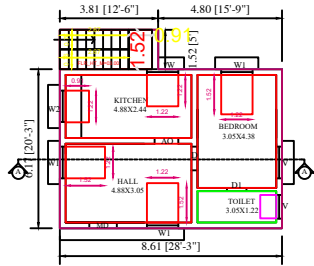
PROPOSED GROUND FLOOR PLAN
