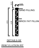
DETAILS OF PERCUSSION PIT
