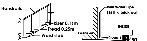
STAIRCASE DETAILS
