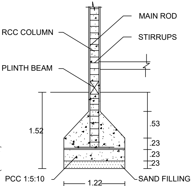
COLUMN DETAILS
