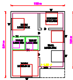
PROPOSED GROUND FLOOR
