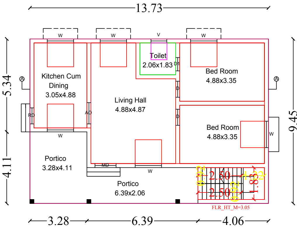
Ground Floor
