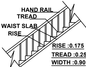
STAIRCASE DETAILS
