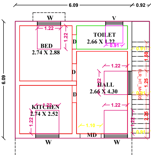
FLOOR-GROUND
