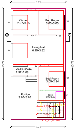
PLAN
