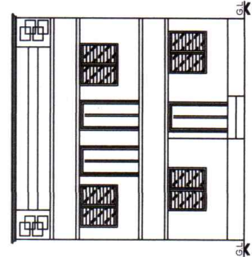
Front Elevation
