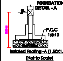
Foundation Not To Scale
