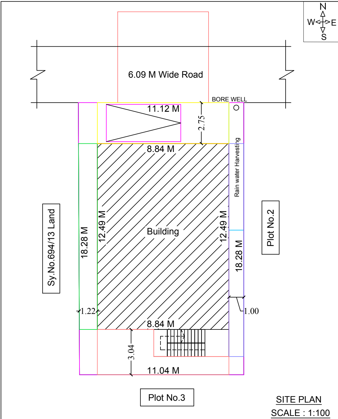
RAIN WATER HARVESTING SYSTEM
