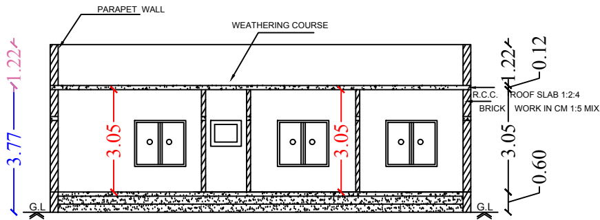
Section on-AA
