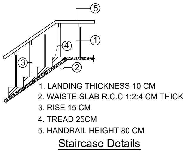
Staircase Details
