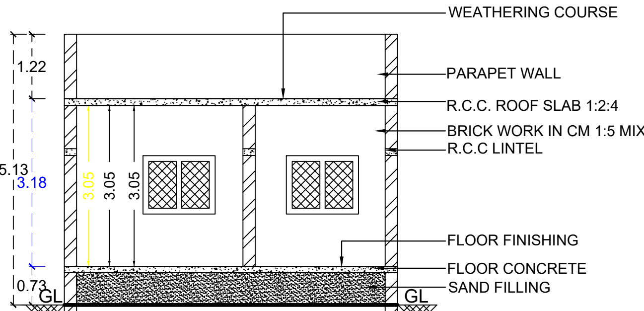
SECTION A1-A1
