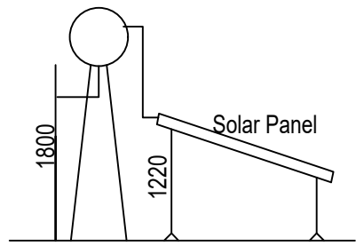
SIDE ELEVATION
