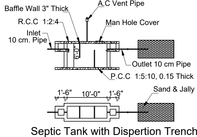
Septic Tank with Dispersion Trench
