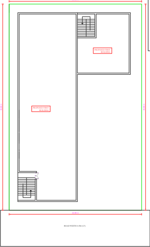
SITE PLAN
