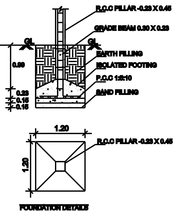
FOUNDATION DETAILS
