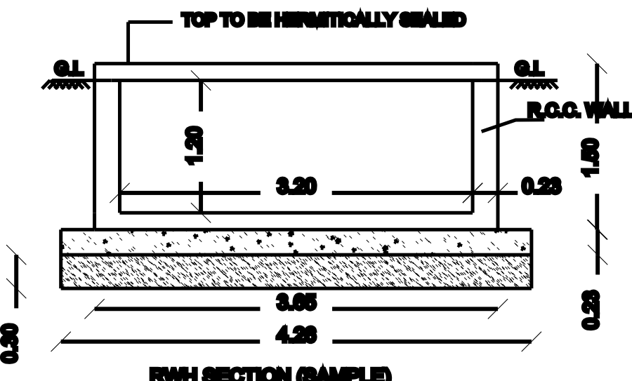
RWH SECTION (SAMPLE)
