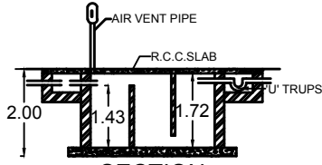
SECTION
