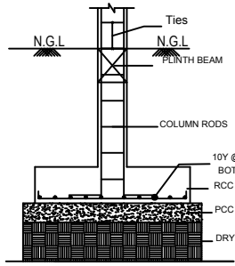
FOUNDATION DETAILS (Concentric Footing)
