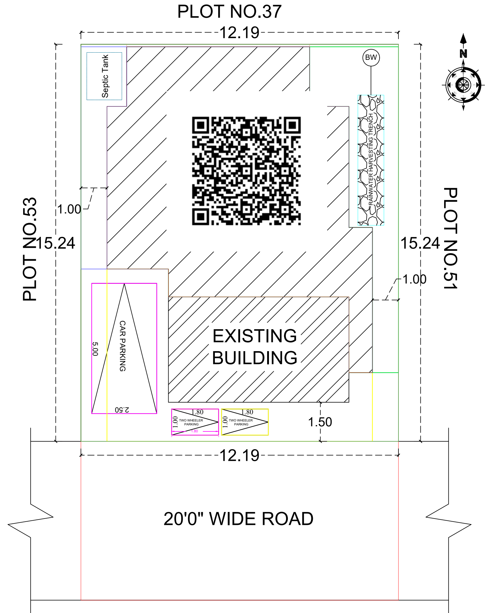
SITE PLAN (1:100)
