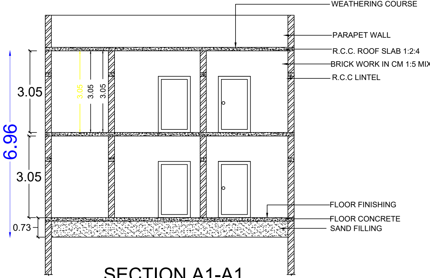
SECTION A1-A1
