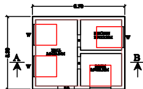
GROUND FLOOR
