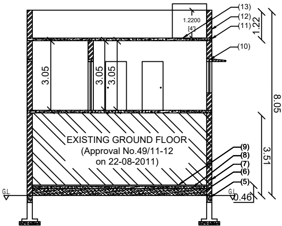
FIRST FLOOR SECTION "AA"
