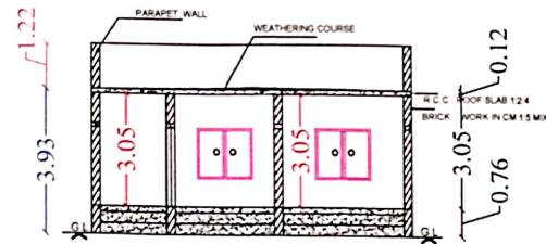
Section on-"AA"
