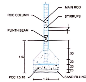
COLUMN DETAILS
