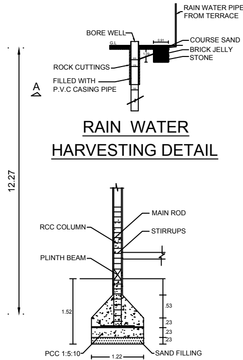
COLUMN DETAILS
