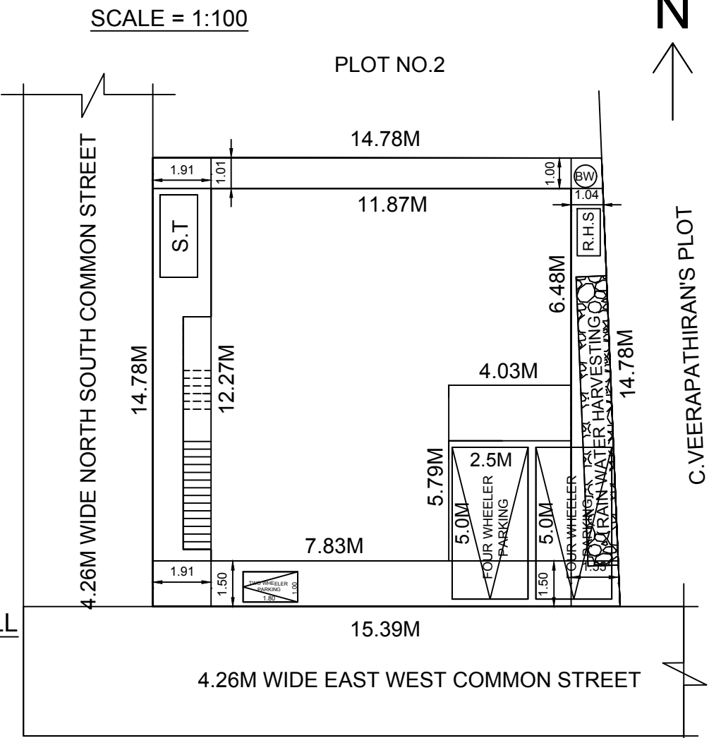
SITE PLAN
