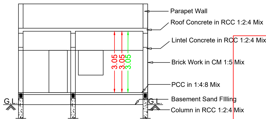
Section RR
