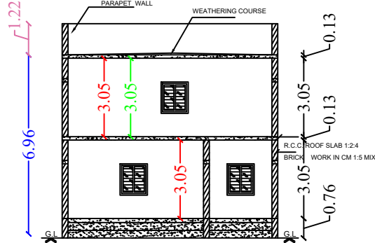
Section on-"AA"
