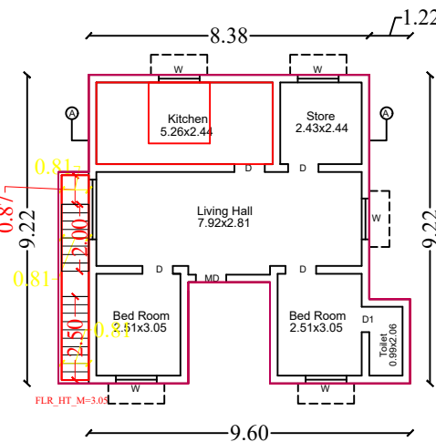
Ground Floor Existing
