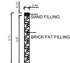
DETAILS OF PERCULATION PIT
