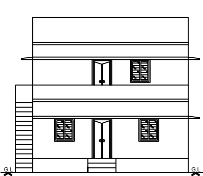
Front Elevation
