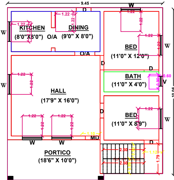
FLOOR-GROUND
