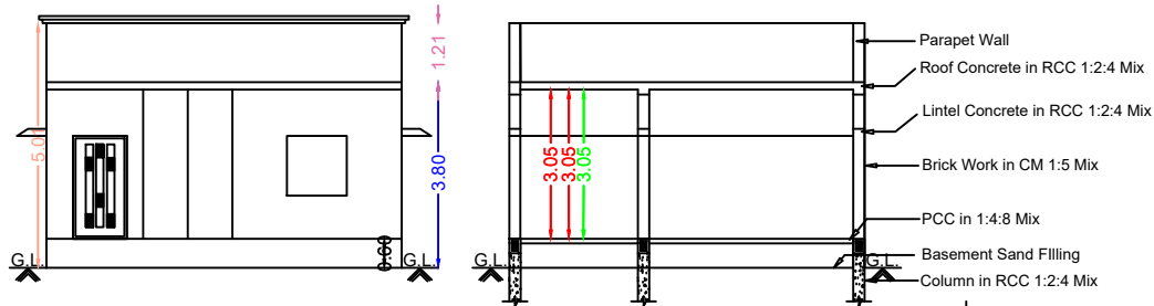
Front Elevation
