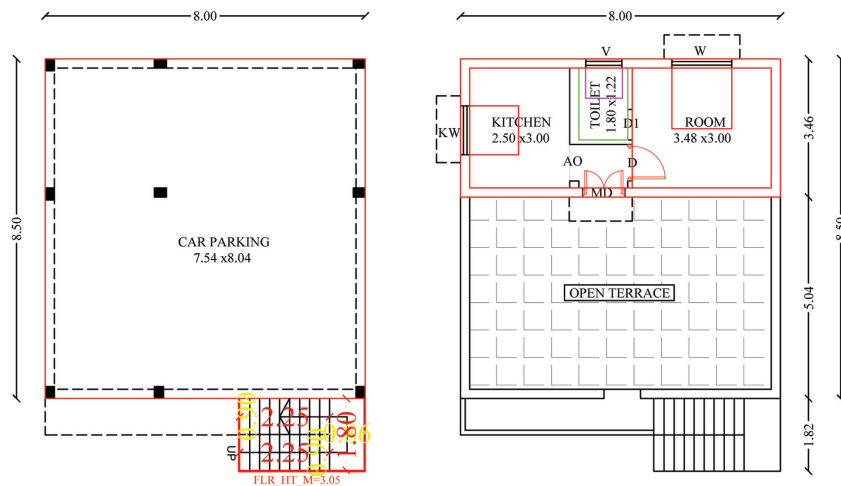
STILT FLOOR PLAN
