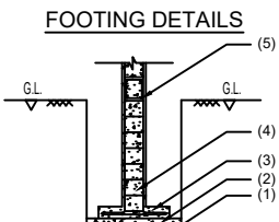
FOOTING DETAILS
