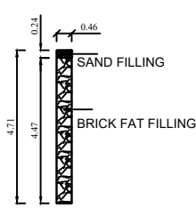
DETAILS OF PERCULATION PIT
