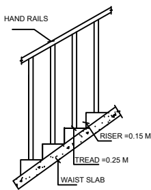
STAIR CASE DETAILS
