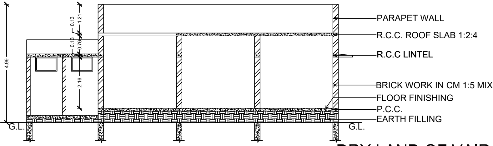
SECTION ON "VR"
