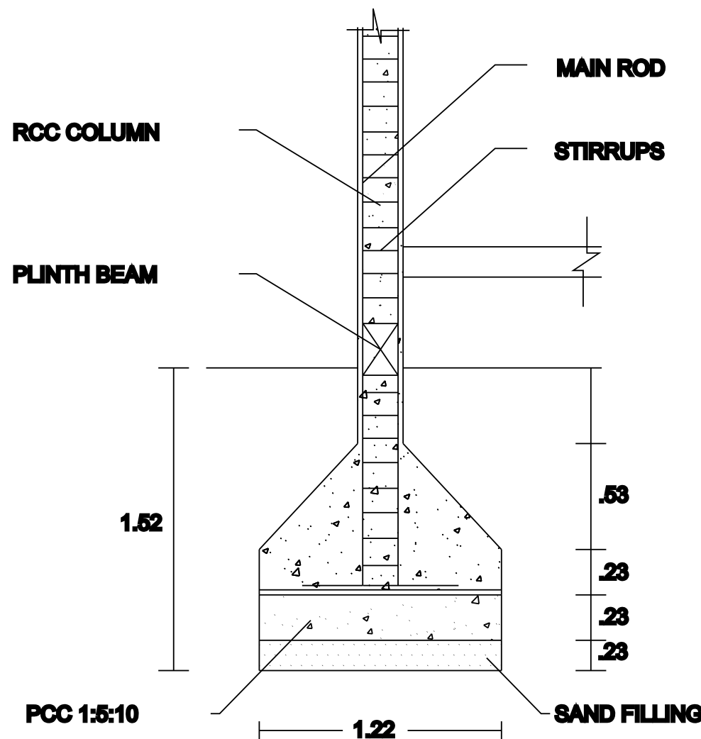
COLUMN DETAILS
