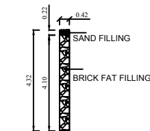
DETAILS OF PERCOLATION PIT
