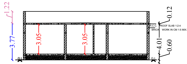
Section on-"AA"
