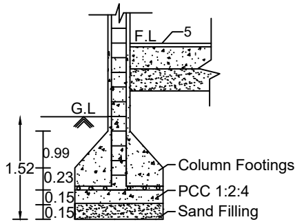
Foundation Details
