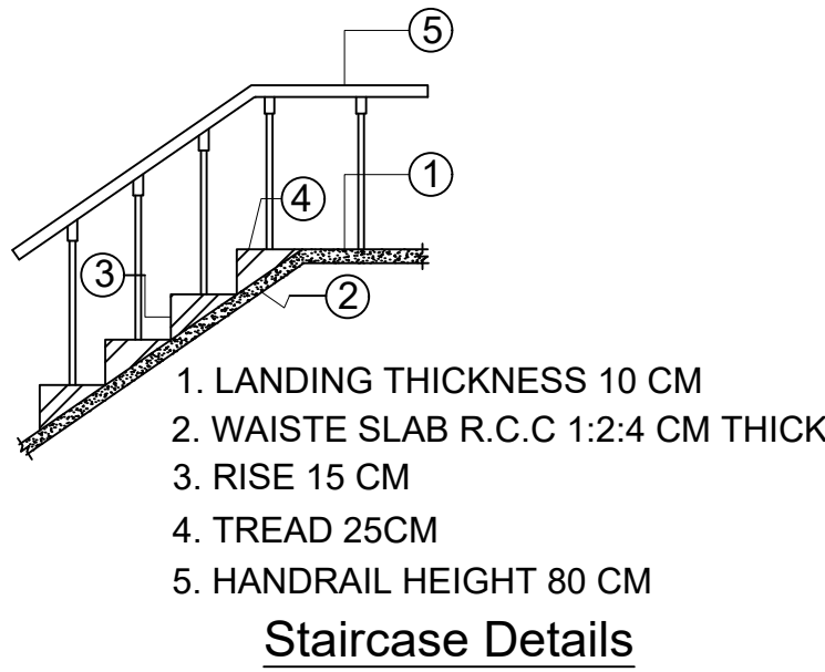
Staircase Details
