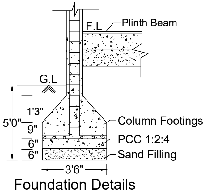
Foundation Details
