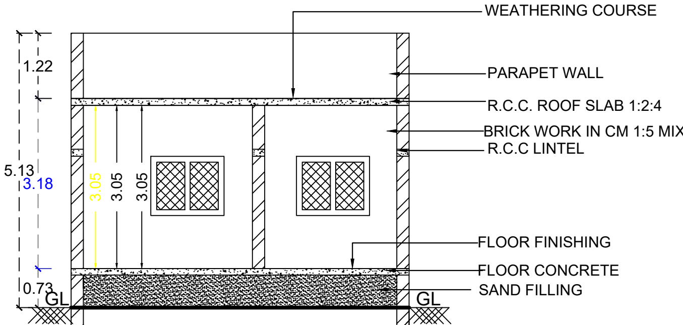
SECTION A1-A1
