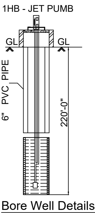
Bore Well Details
