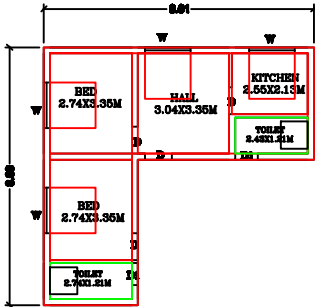
OUT HOUSE PLAN
