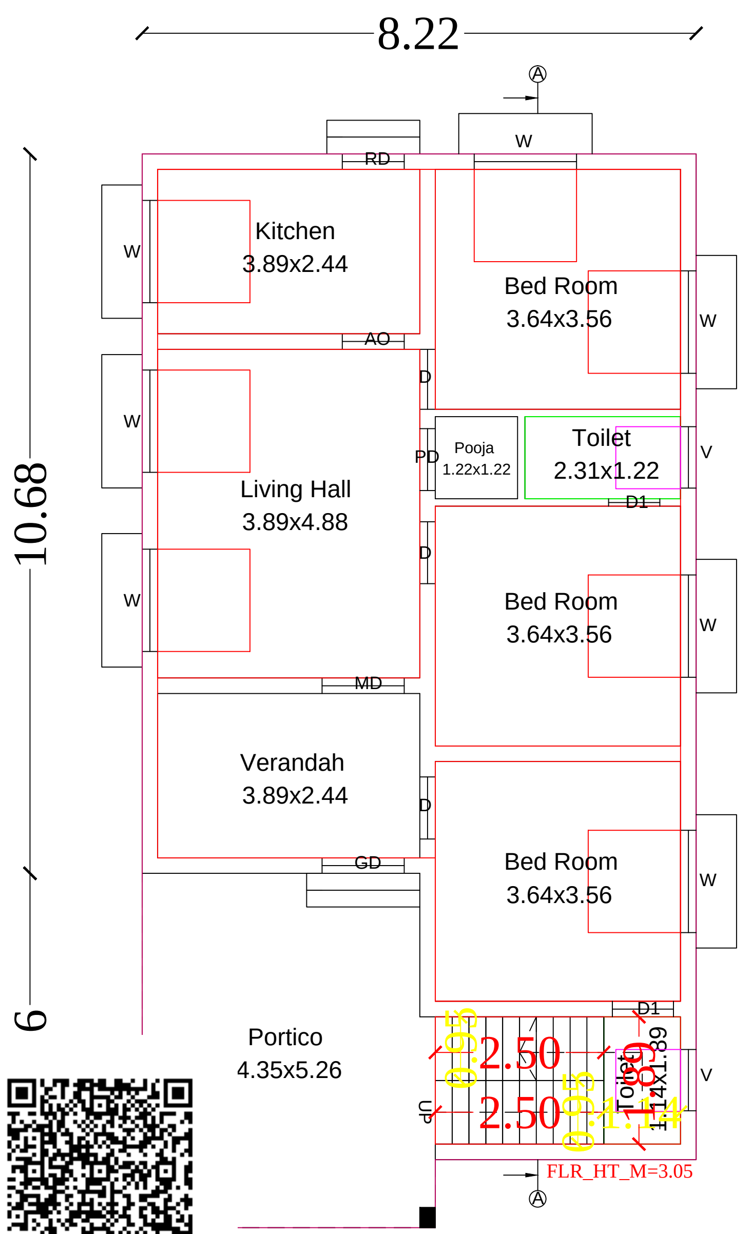
Ground Floor
