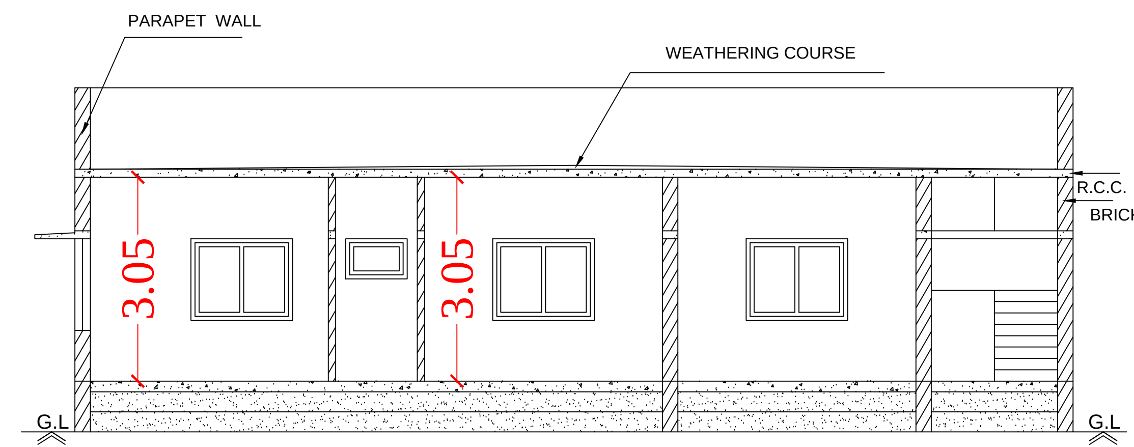
Section on-"AA"
