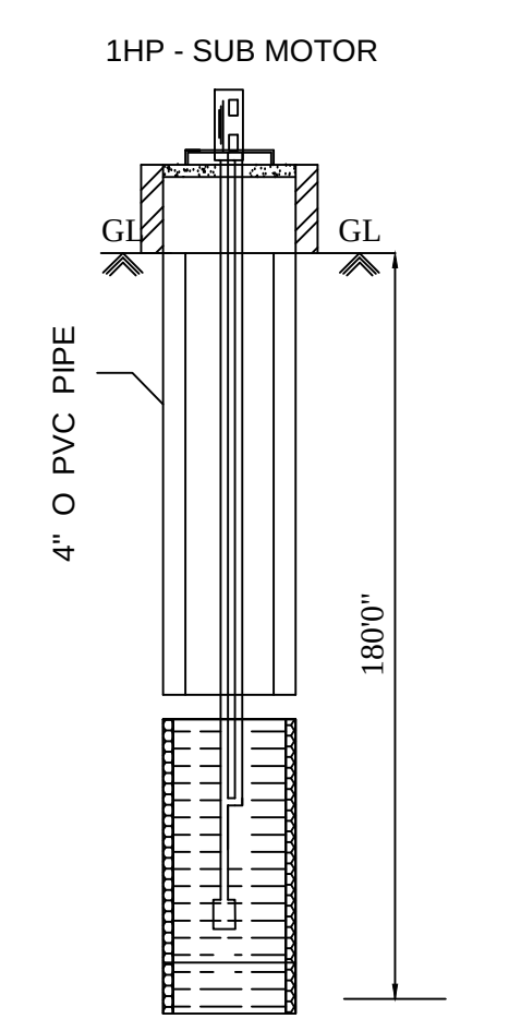
Bore Well Details
