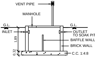
SECTION OF SEPT.TANK
