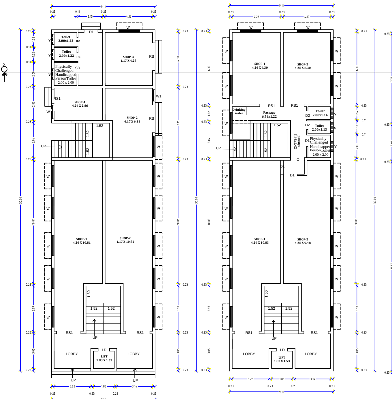
TYPICAL FIRST AND SECOND FLOOR PLAN TYPICAL_FLOOR_PLAN=1,2
