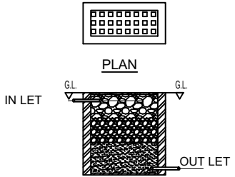
RAINWATER STORAGE PIT DETAILS
