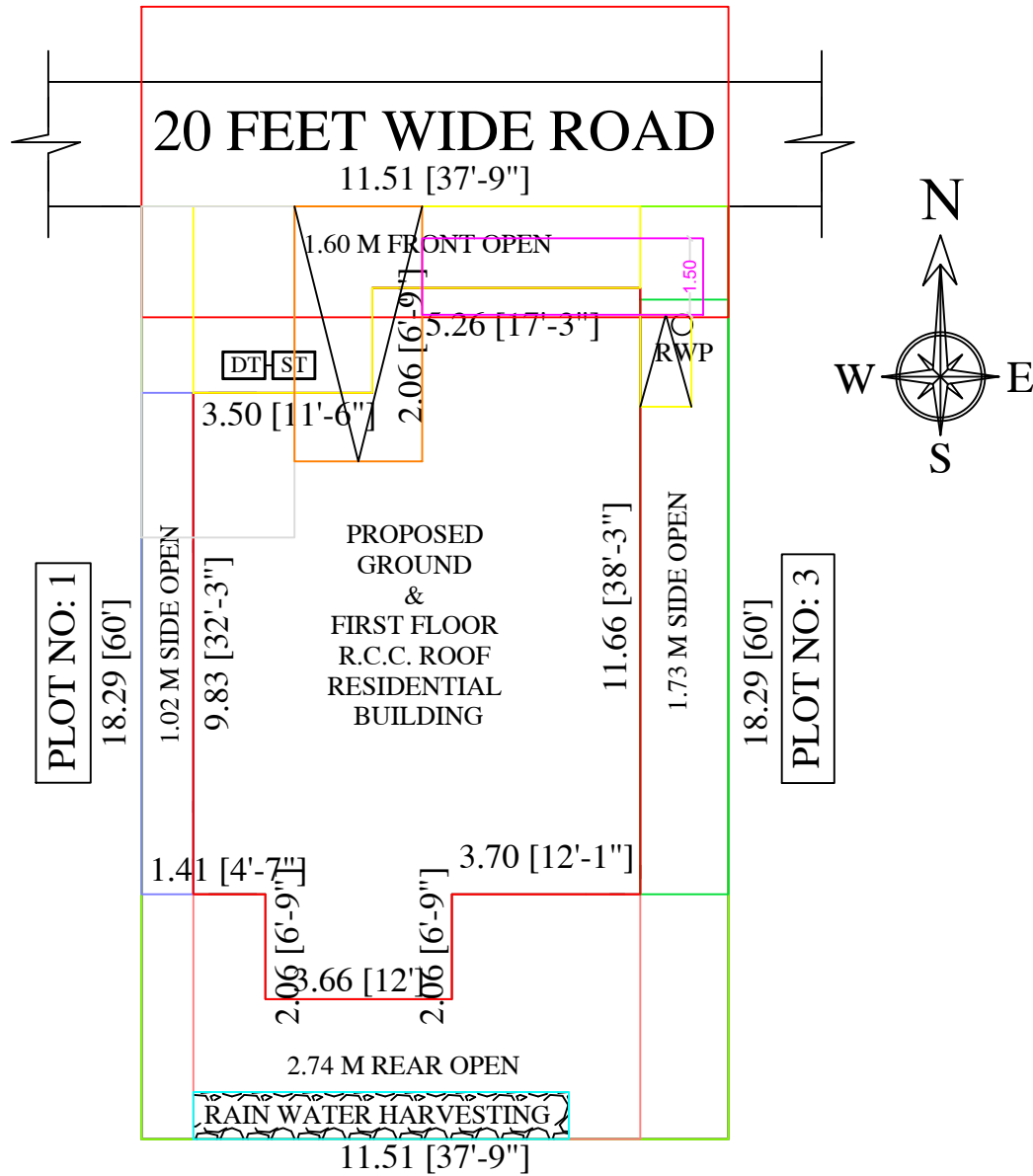
SITE PLAN
