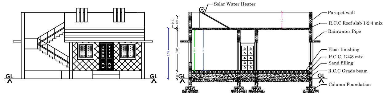
FRONT ELEVATION
