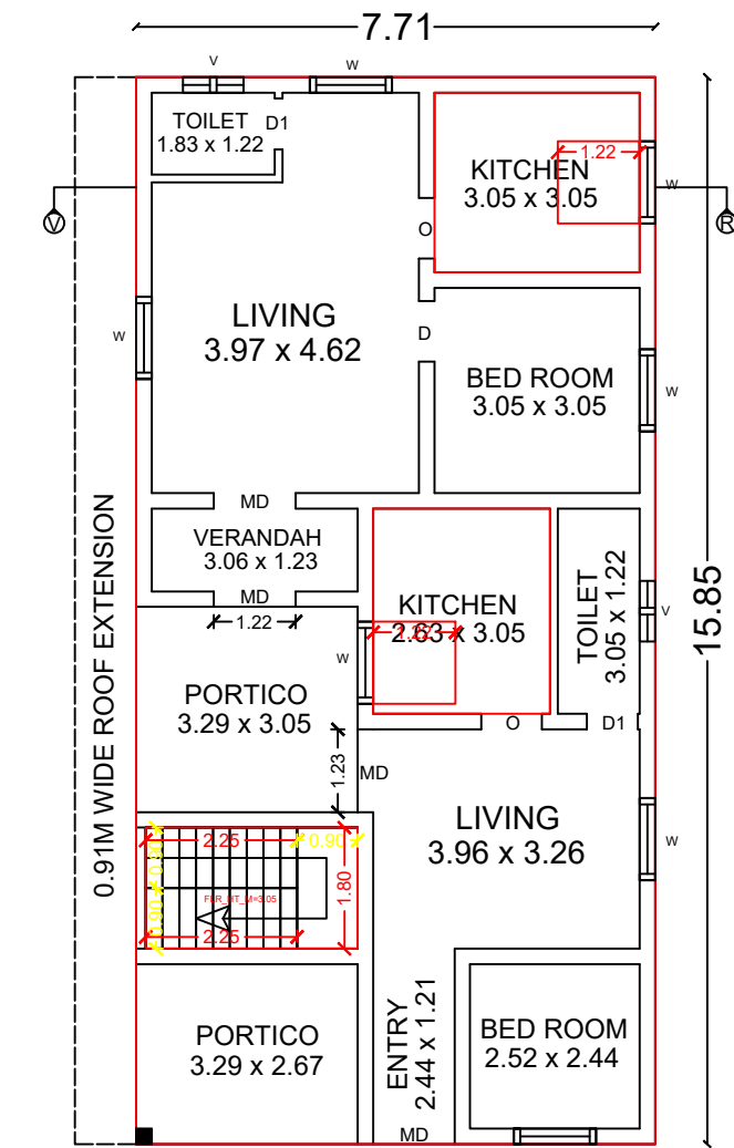
EX. GROUND FLOOR PLAN
