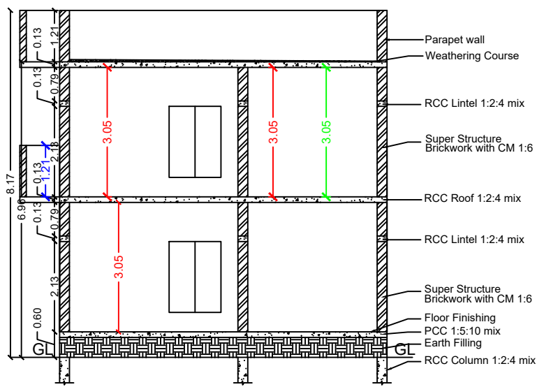
SECTION ON "VR"
