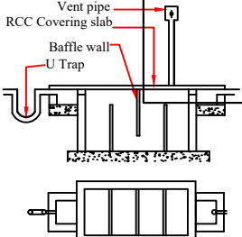
SEPTIC TANK
