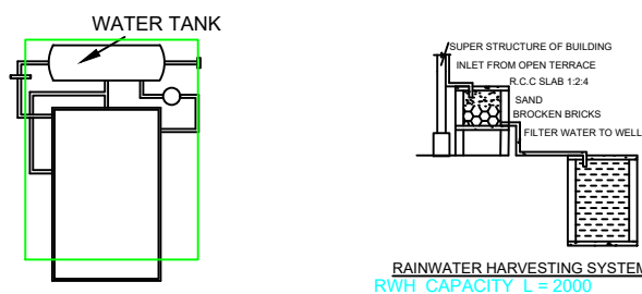
Section RR
