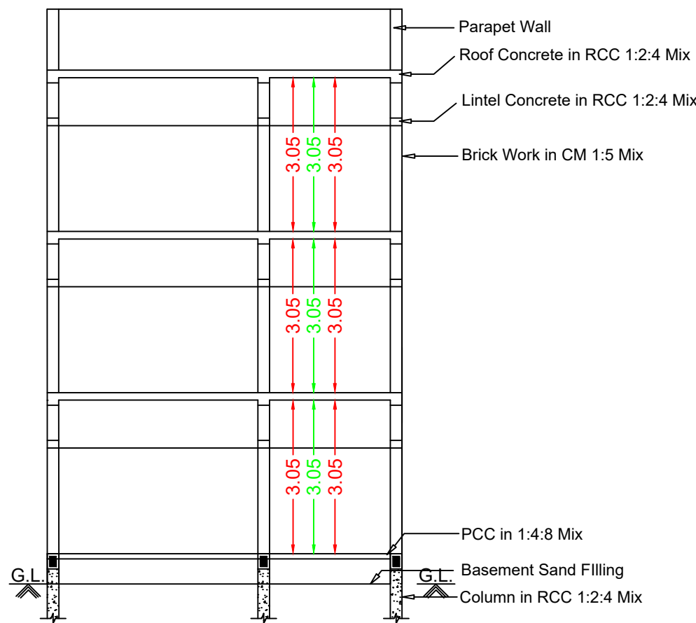
Section RR
