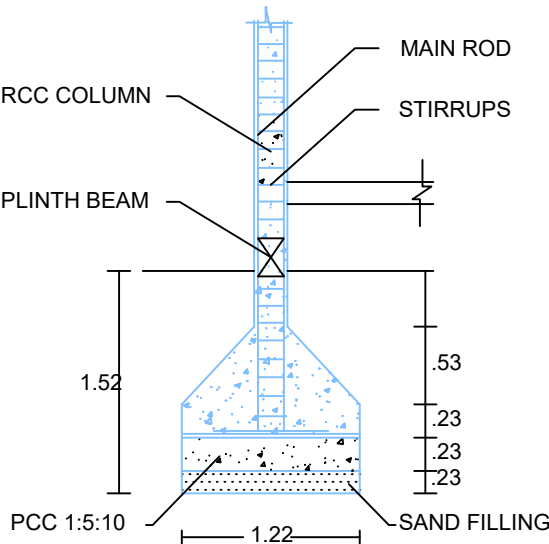
COLUMN DETAILS
