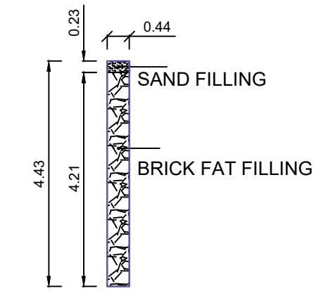
DETAILS OF PERCULATION PIT
